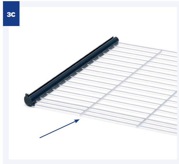
Slide the 2 lower side panels (c) into the profiles. Again, make sure the vertical wires are facing outwards.
